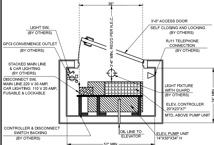
MACHINE ROOM PLAN NTS
