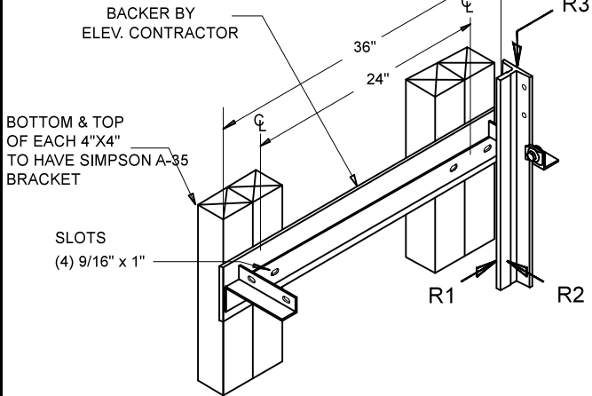
RAIL BRACKET & RAIL FORCES NTS
